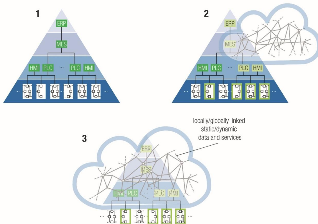
Figure 3 Gradually replacement of the classical automation pyramid (VDI/VDE 2013)
